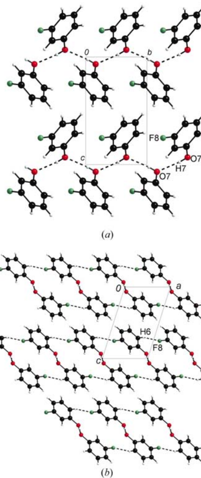
Figure 2 ( a ) Crystal structure of 3-fluorophenol at 150 K viewed down the a axis. 3-Fluorophenol crystallizes with one molecule in the asymmetric unit in the space group P2_1 , thereby forming a chain motif adopted by smaller alcohols. ( b ) Close contacts formed between H6...F8 of different chains (these contacts are omitted in Fig. 2 a for clarity). Colour scheme: C black, F sea green, H light turquoise, O red.
