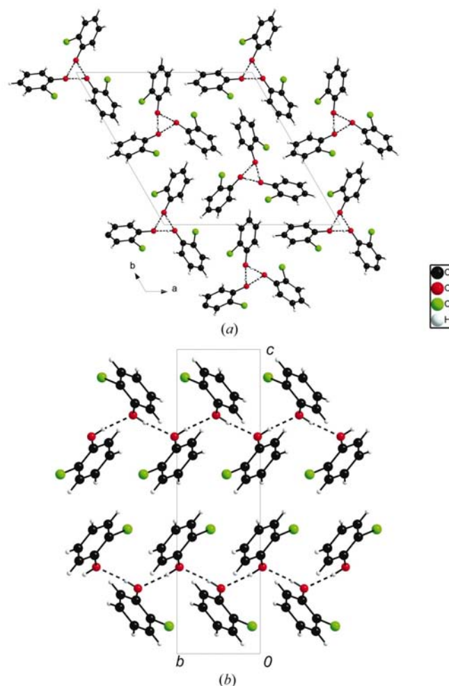
Figure 1 (a) Crystal structures of 2-chlorophenol at ambient pressure and 100 K. Helices are formed about 3_2 axes by OH...OH hydrogen-bond formation. (b) The crystal structure of 2-chlorophenol at 0.12 GPa. The application of pressure changes the behaviour of the chlorophenyl substituent so that chains are formed where molecules are related by a 2_1 screw axis. Colour scheme: C black, Cl green, H light turquoise, O red.
